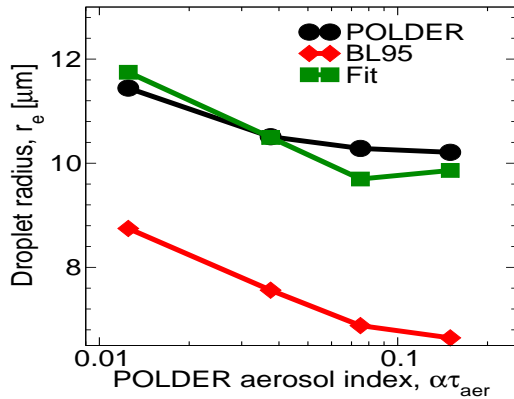
Figure 1. Relationship between cloud droplet effective radius ( \mu\text{m} ) and aerosol index for POLDER observations (line) and for the LMDZ model with the original [Boucher and Lohmann, 1995] “D” formula (dash-dot) and with the adjusted formula (dash).
