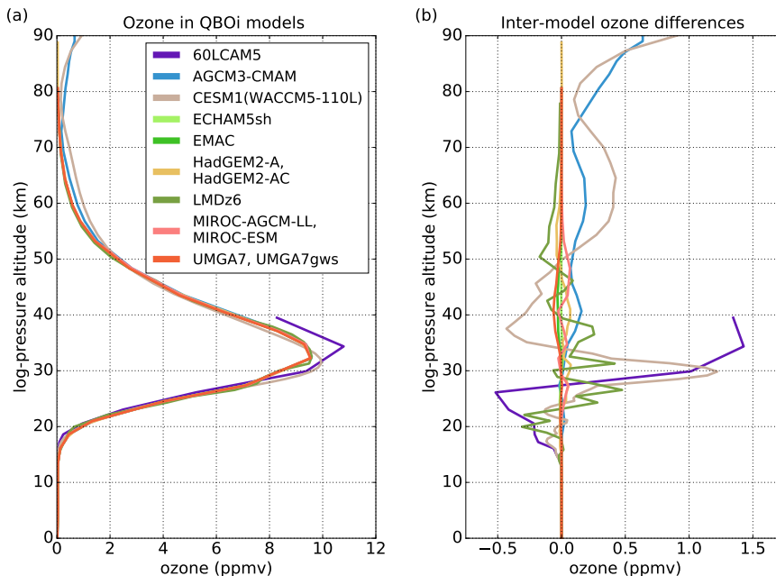
Figure 6. (a) Vertical profiles in the tropics of the ozone concentration prescribed in QBOi timeslice experiments (Experiments 2–4; Table 5 indicates which models have performed these experiments), for models that do not include ozone chemistry (as indicated in Table 8). Each vertical profile is an average over the 5^{\circ}\text{S} – 5^{\circ}\text{N} latitude band, zonal mean, and annual mean. (b) As (a), but showing differences from a reference profile so that inter-model variations are more clearly visible. The reference profile is the 1988–2007 climatology of the SPARC ozone referred to in Appendix A (item A1). The period 1988–2007 is the same as that recommended for Experiment 2 for the SST and sea ice climatologies (Appendix A, item A2).
