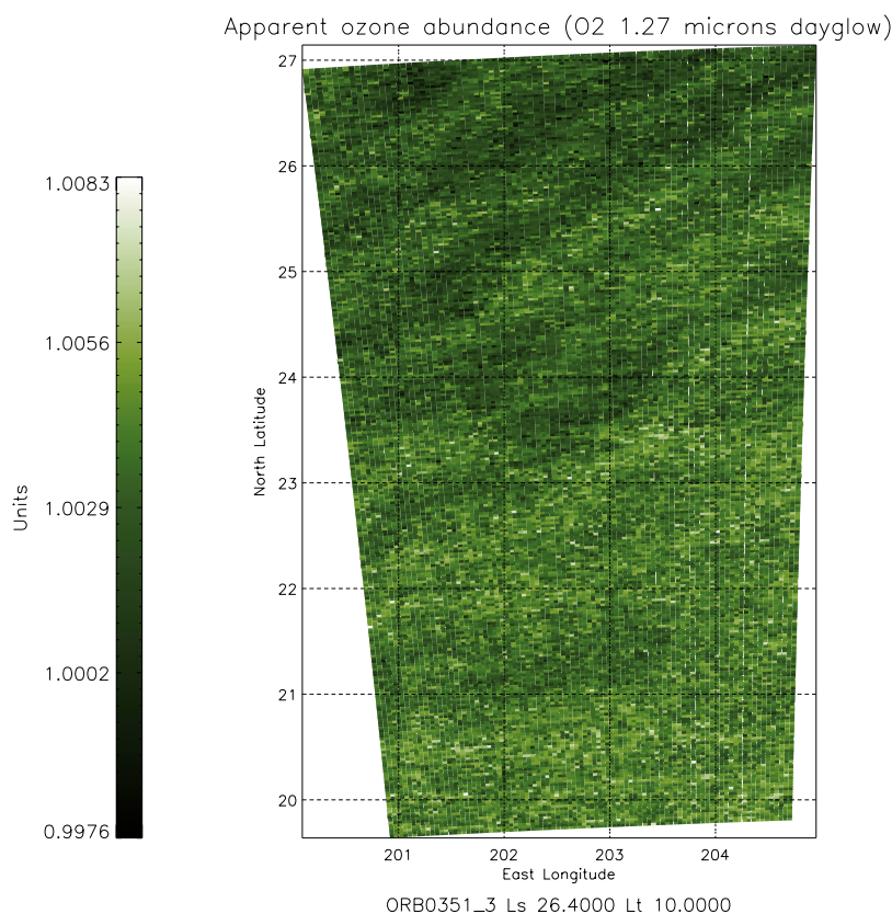
Figure 8. The 1.27 \mu\text{m} O 2 emission OMEGA map. The displayed variable is the ratio between the reflectance at 1.271 \mu\text{m} (O 2 emission) and the mean reflectance at 1.256 \mu\text{m} and 1.285 \mu\text{m} (continuum). This variable indicates the concentration of the passive tracer O 3 above 20 km. The method used in this map is described by Zasova et al. [2006] and was provided as a personal communication by F. Altieri (2006).
