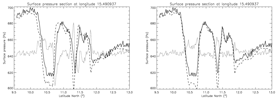
Figure VI.8: [LEFT] Meridional section of surface pressure fields in the ORB0278.3 case prior to any registration shift correction. The OMEGA surface pressure field (full line) is slightly shifted from the reference surface pressure field based on MOLA (dashed line). As a result, the OMEGA leveled surface pressure field (dotted line) features artificial high/low values in the vicinity of the highest topographical gradients. [RIGHT] Same figure, after the registration shift correction.
