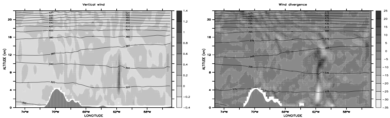
Fig. 14. Case 2: Results of the WRF simulations. Longitude-altitude cross sections at latitude -29.45^{\circ}\text{N} . Left: Vertical wind velocity ( \text{m s}^{-1} ) and isentropes (K). Right: Horizontal wind divergence ( \text{s}^{-1} ) and isentropes (K).
