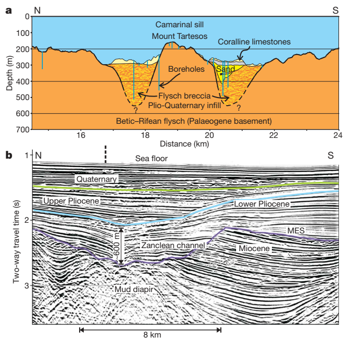
Figure 2 | Evidence for an erosion channel across the Gibraltar Strait.
