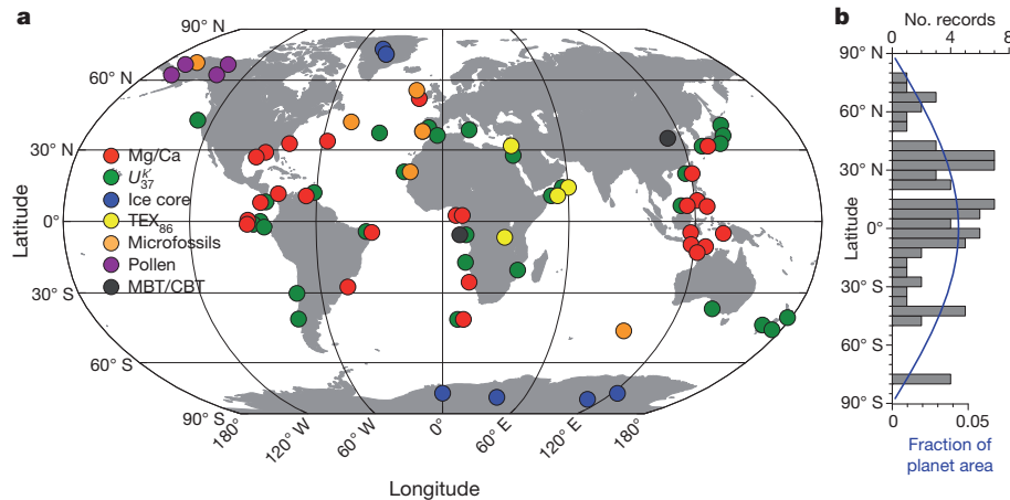
Figure 1 | Proxy temperature records. a , Location map. CBT, cyclization ratio of branched tetraethers; MBT, methylation index of branched tetraethers; TEX 86 , tetraether index of tetraethers consisting of 86 carbon atoms;
