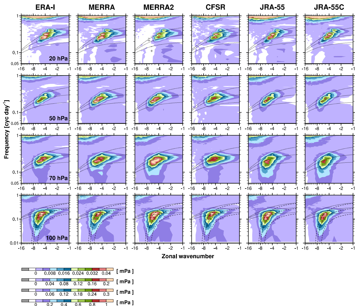
Figure 10. The same as in Fig. 9 but for F_z of anti-symmetric modes. The MRG wave dispersion curves for the windless background state are indicated by dotted for h = 8, 60, and 480 m. At 100 hPa, the dispersion curves for the background zonal wind of +10 m s ^{-1} are also indicated (dashed).
