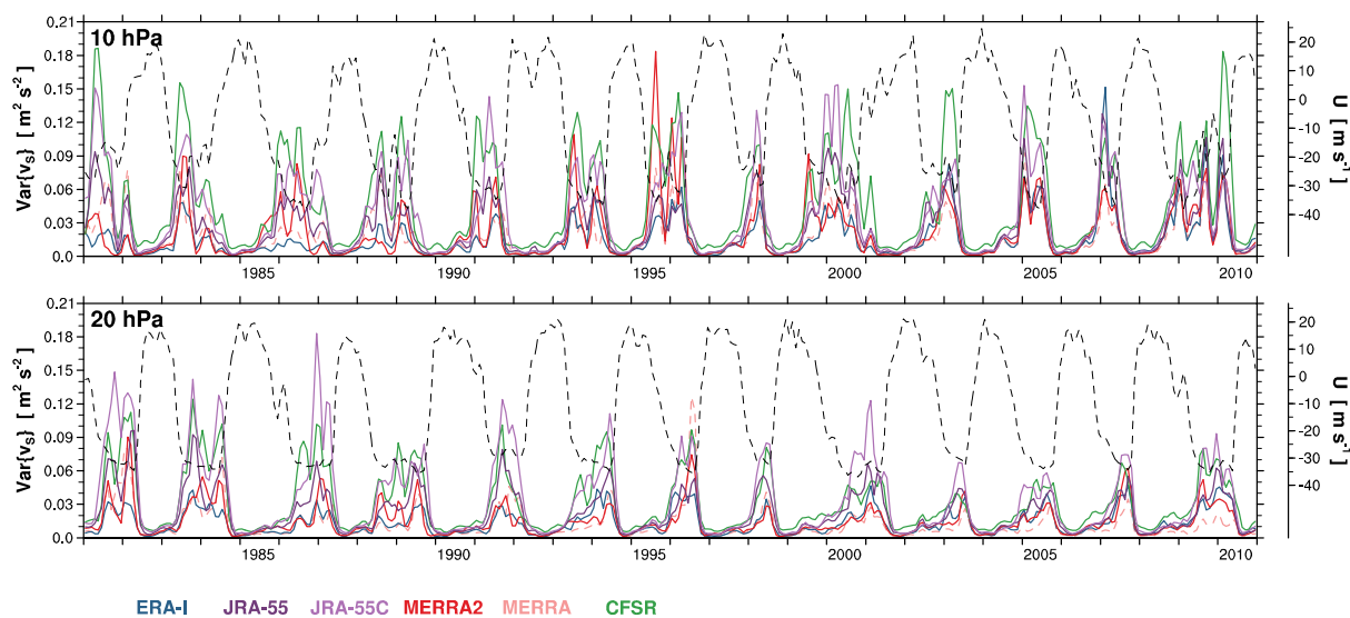
Figure 12. Monthly time series of variances of the symmetric component of meridional wind at (upper) 10 and (lower) 20 hPa, filtered for 0.5 < \omega < 0.7 \text{ cyc day}^{-1} with k = -7 and 0.6 < \omega < 0.75 \text{ cyc day}^{-1} with k = -8 (see Fig. 2). The monthly zonal wind from radiosonde observations is also presented at each level (dashed black).
