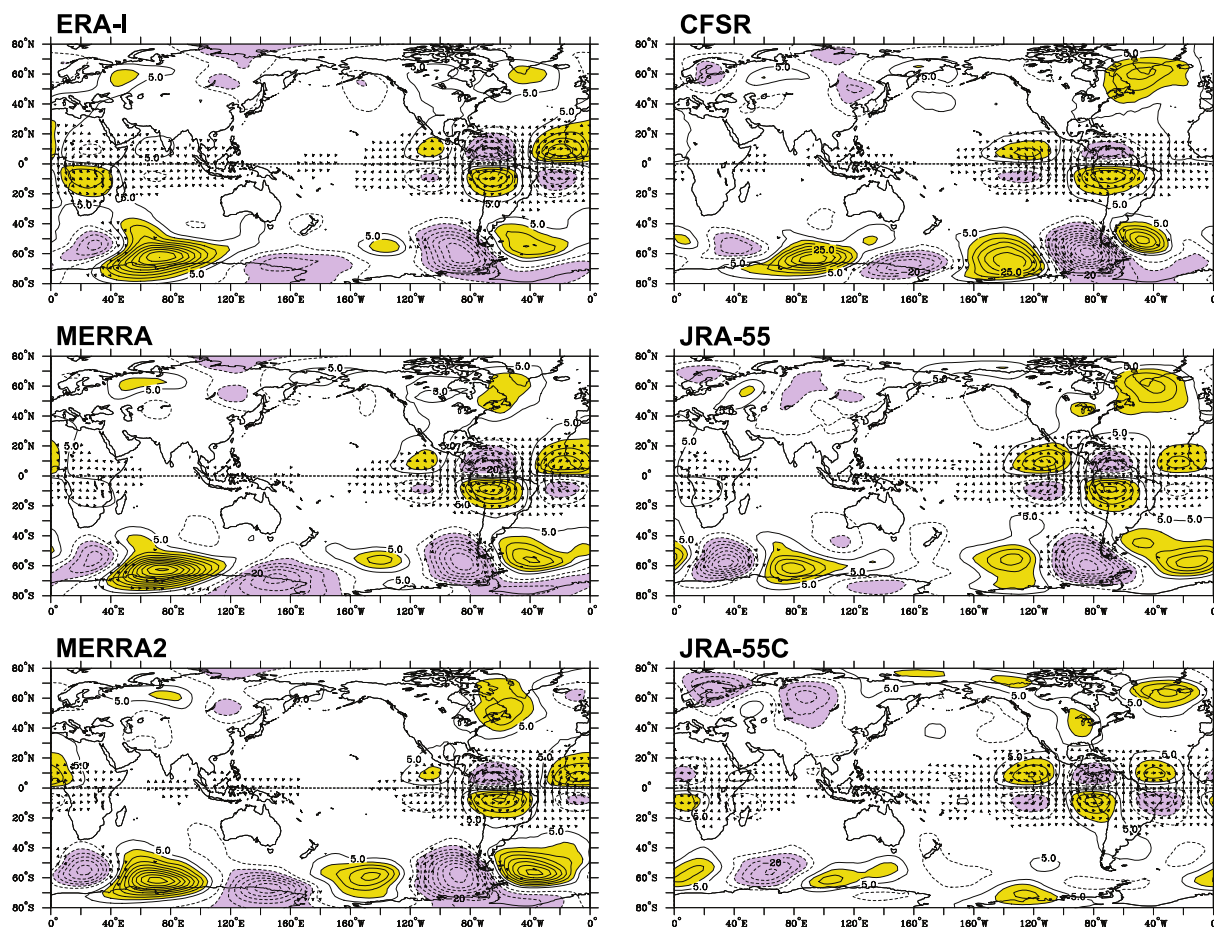
Figure 5. The same as in Fig. 4 except for MRG waves. The EOFs for MRG waves are calculated using 2–6 day filtered meridional winds.
