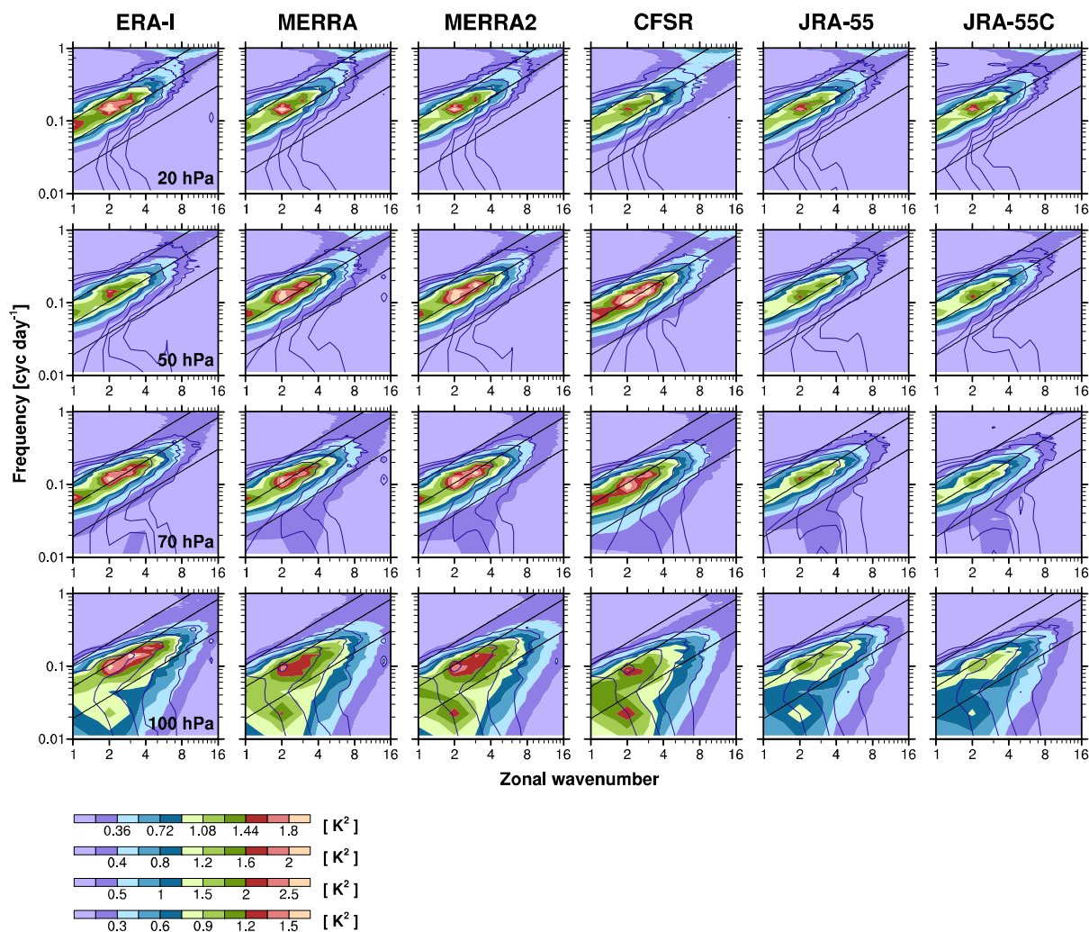
Figure 1. Zonal wavenumber–frequency power spectra of the symmetric component of temperature at 100, 70, 50, and 20 hPa (from bottom to top) from the standard-level datasets of six reanalyses (ERA-I, MERRA, MERRA-2, CFSR, JRA-55, and JRA55-C: from left to right), averaged over 15°N–15°S in 1981–2010. The power spectra are presented in the variance-preserving form with log-scale axes. The Kelvin wave dispersion curves are indicated by black solid for the equivalent depths ( h ) of 8, 60, and 240 m. The ratio of the spectral power to that of the background spectrum is indicated by thin purple for the values of 1.5, 2, 3, and 5.
