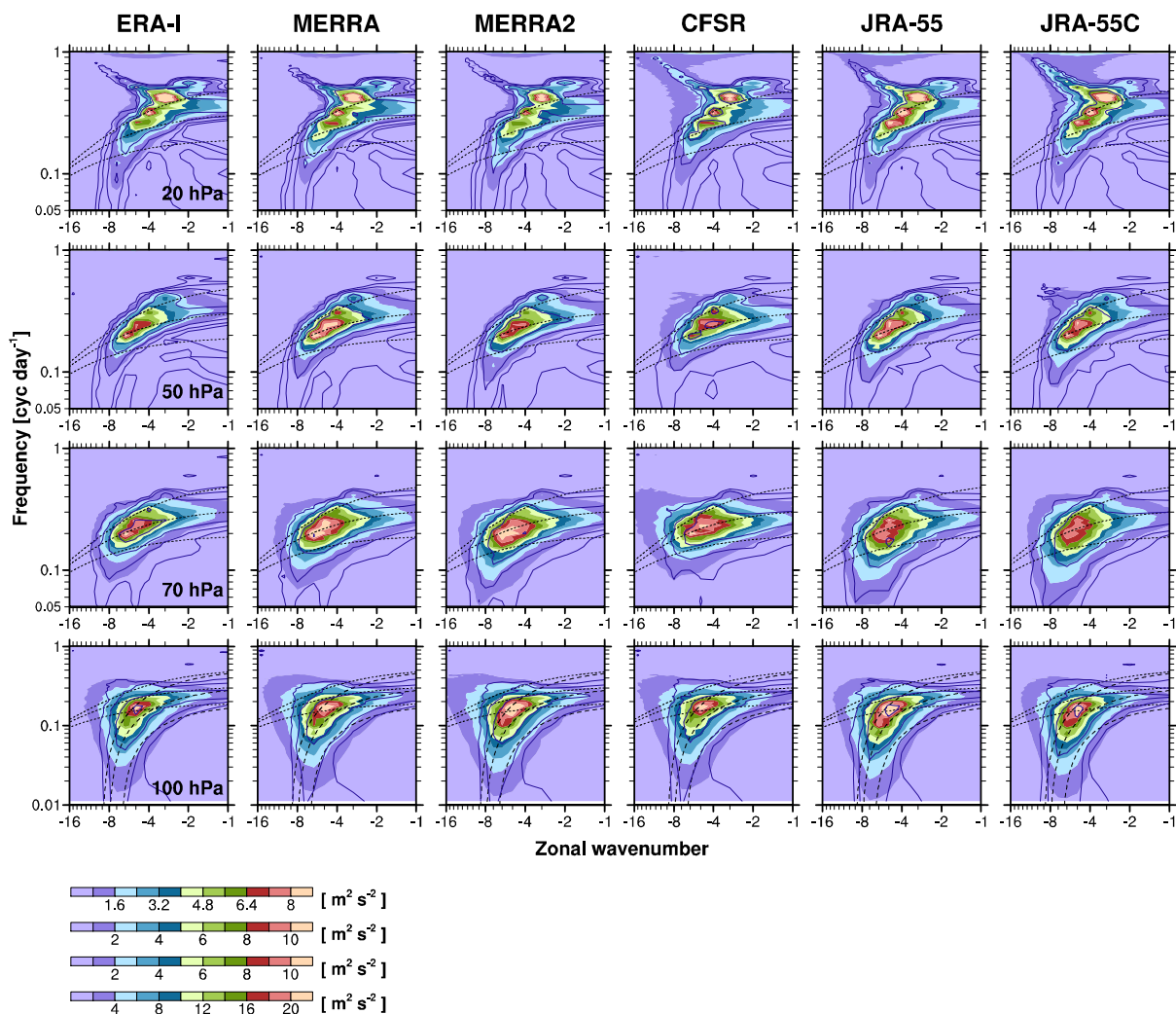
Figure 2. The same as in Fig. 1 except for the spectra of the symmetric component of meridional wind. The mixed Rossby-gravity (MRG) wave dispersion curves for the windless background state are indicated by dotted for h = 8, 60, and 480 m. At 100 hPa, the dispersion curves for the background zonal wind of +10 \text{ m s}^{-1} are also indicated (dashed).
