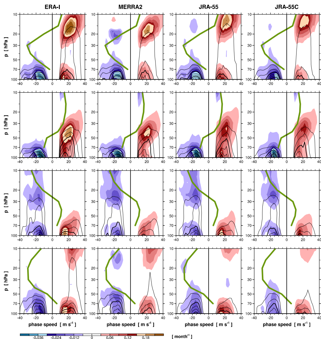
Figure 11. Vertical profiles of phase-speed spectra of the EP flux divergence (shading) and vertical EP flux (black contour) for the Kelvin waves at c > 0 and MRG waves at c < 0 , composited for the QBO phases of maximum westerly tendencies at 20 and 50 hPa (the first and second rows, respectively) and easterly tendencies at 20 and 50 hPa (the third and last rows, respectively), from the model-level datasets of ERA-I, MERRA-2, JRA-55 and JRA-55C. The zonal wind profiles for those composites are also indicated (green; see the text for the composite method). The contour intervals of the EP flux are 0.005 and 0.0005 \text{mPa} / \text{m s}^{-1} for the Kelvin and MRG waves, respectively, and every third contour is distinguished by thicker lines.
