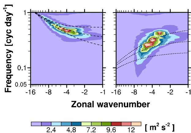
Figure 13. The same as in Fig. 2 (rightmost in the first row) except for the average over the months when (left) the zonal wind U < -25 \text{ m s}^{-1} and (right) U > -20 \text{ m s}^{-1} , at 20 hPa in JRA-55C. The dashed in the left panel indicate the MRG wave dispersion curves for h = 8, 60, and 480 \text{ m} for the background wind of -30 \text{ m s}^{-1} , and the dotted in the right indicate those for the windless background state.
