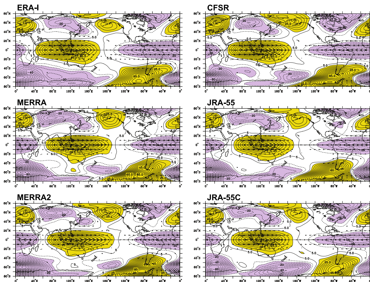
Figure 4. Horizontal wind (arrow) and geopotential perturbations (shading) projected onto the principle component times series of the first EOF modes for Kelvin waves at 50 hPa in each reanalysis. The EOFs for Kelvin waves are calculated using 2–25 day filtered eastward-propagating zonal winds (see the text). The winds are shown at the locations where they are statistically significant.
