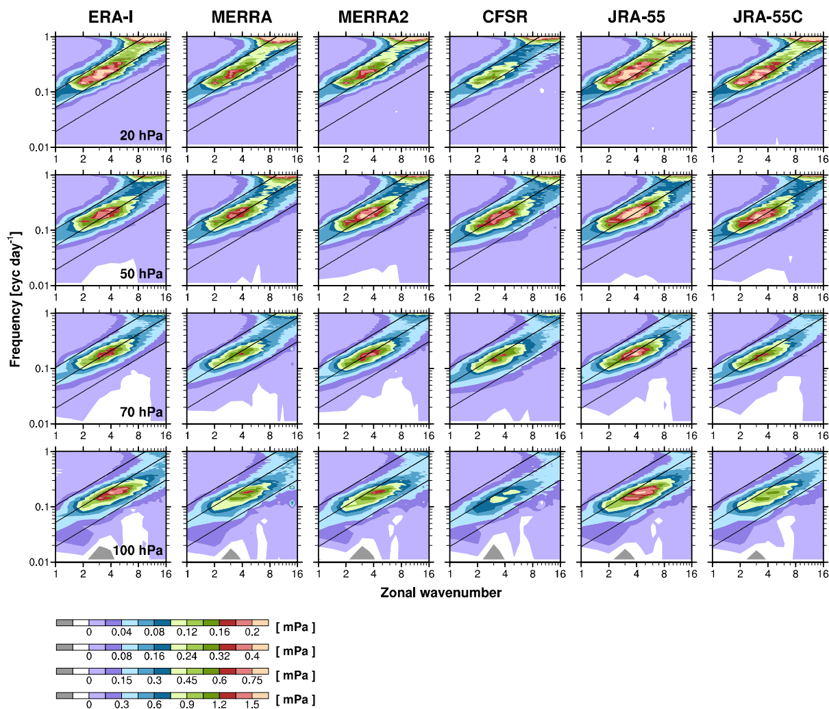
Figure 9. Zonal wavenumber–frequency spectra of the vertical EP flux, multiplied by -1 ( -F_z ), for symmetric modes at 100, 70, 50, and 20 hPa (from bottom to top) from the standard-level datasets of six reanalyses (ERA-I, MERRA, MERRA-2, CFSR, JRA-55, and JRA55-C: from left to right), averaged over 15^\circ\text{N} – 15^\circ\text{S} in 1981–2010. The Kelvin wave dispersion curves are indicated by black solid for h = 8, 60, and 240 m.
