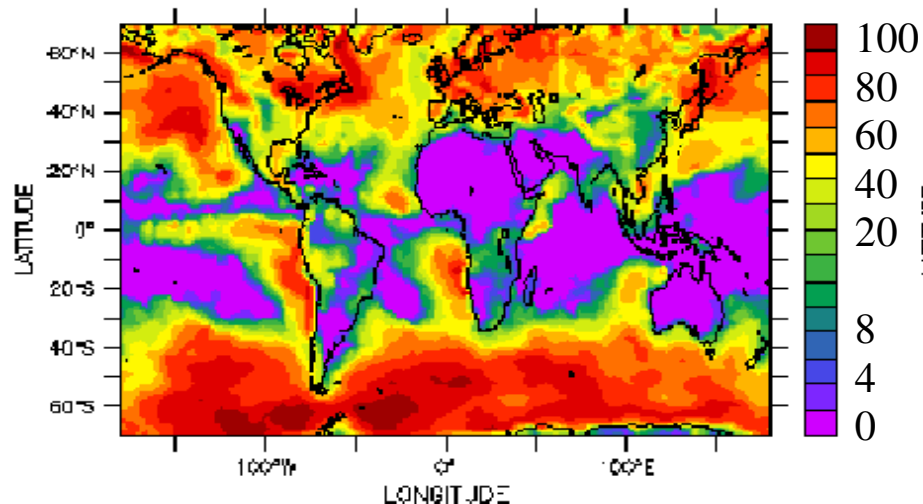
LMDz standard version
