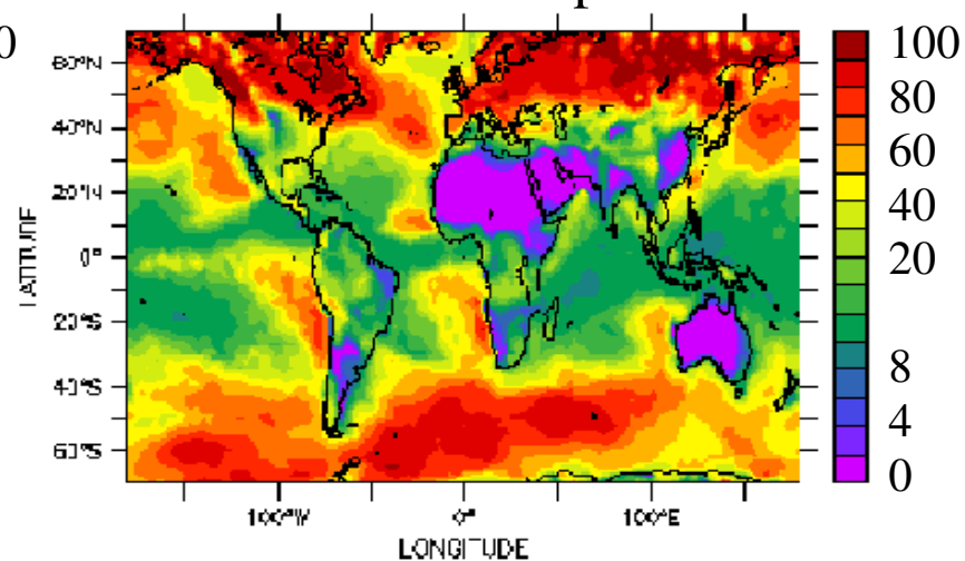
LMDz with thermal plume model
