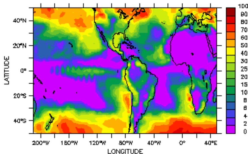
Low level clouds (%), STD phys.
