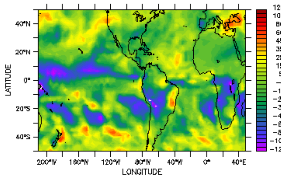
Surf. Down SW radiation (W/m2), NEW-STD
