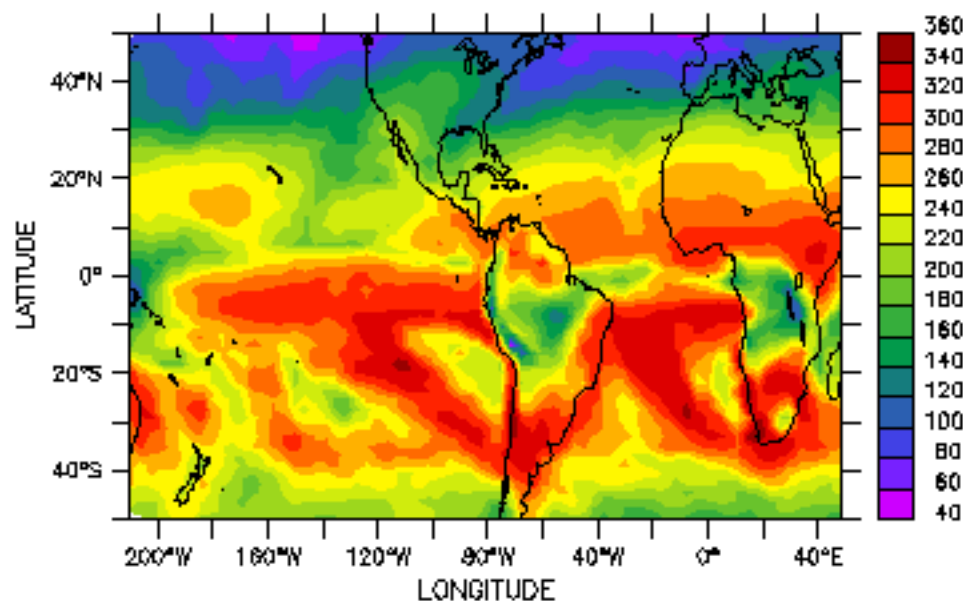
Surf. Down SW radiation (W/m2), STD
