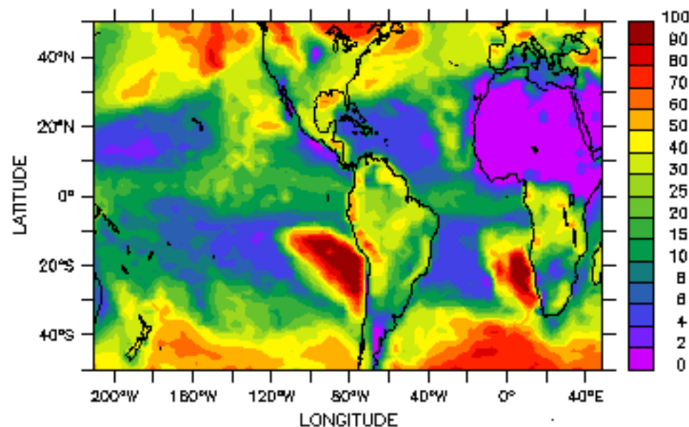
Low level clouds (%), NEW phys.
