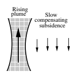
Asymmetric Convective Model of Pleim and Chang 1992
