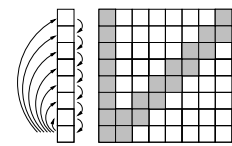
Asymmetric Convective Model of Pleim and Chang 1992
