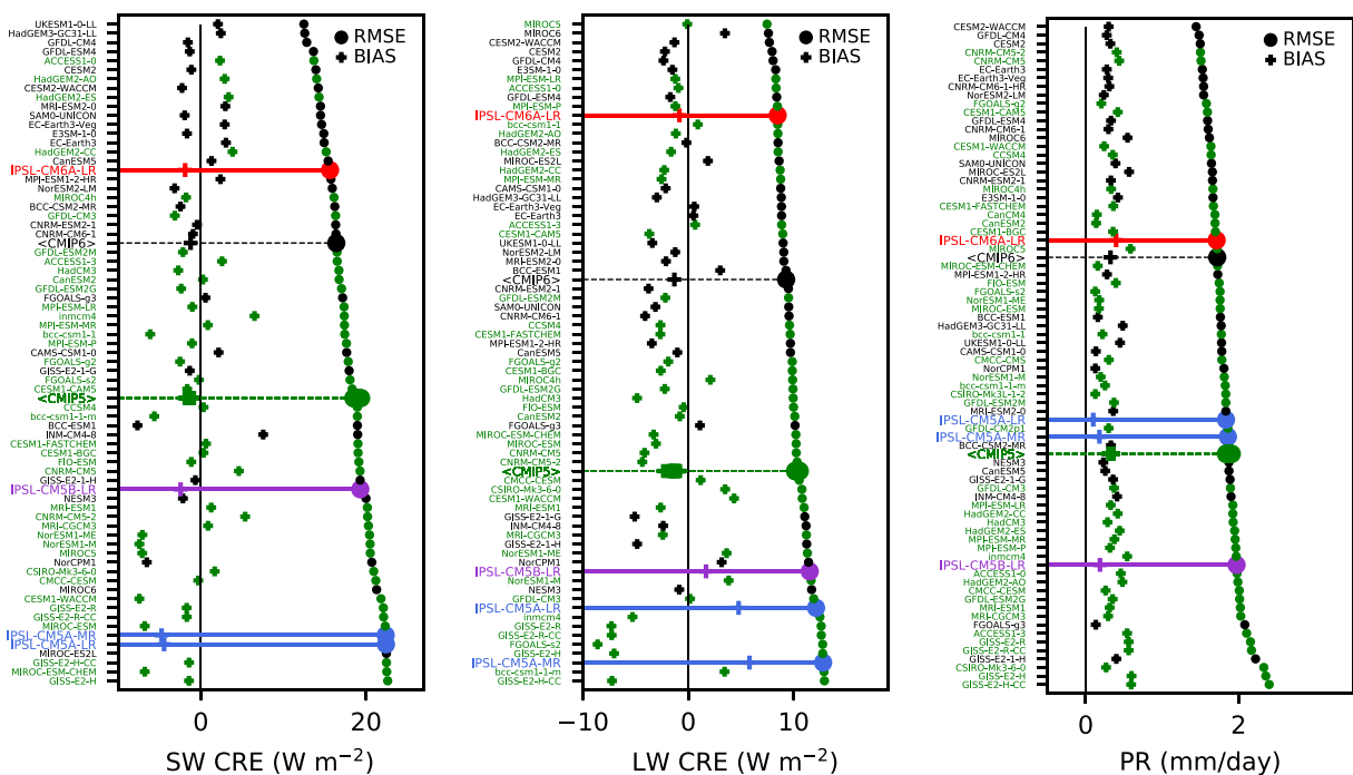
Figure 19. Same as Figure 18 but for the shortwave cloud radiative effect (SW CRE, in W m -2 ), longwave cloud radiative effect (LW CRE, in W m -2 ), and precipitation (PR, in mm day -1 ). The RMSE and biases are computed against the radiative fluxes from CERES-EBAF and precipitation from GPCP.
