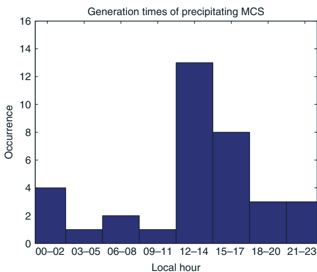
Figure 6. Histogram of the local times of generation of the precipitating MCSs detected over the rain-gauge network in August–September 2006. This figure is available in colour online at wileyonlinelibrary.com/journal/qj
