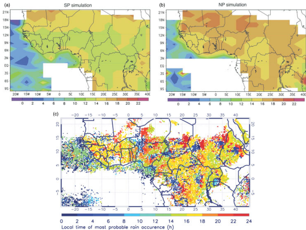
Figure 14. Most probable local times of precipitating events for (a) SP and (b) NP LMDZ simulations and (c) TMPA data.
