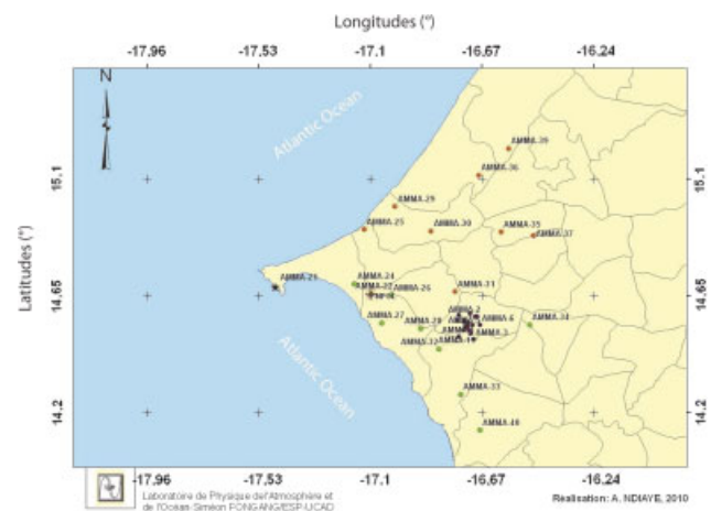
Figure 1. Geographical map showing the rain-gauge network in Senegal. This figure is available in colour online at wileyonlinelibrary.com/journal/qj
