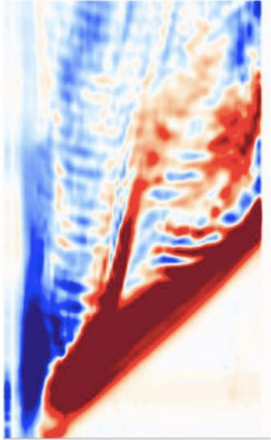
SSH at the equator
