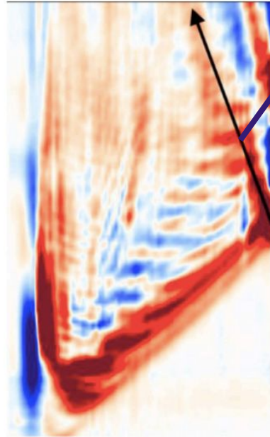
SSH at 4°N
