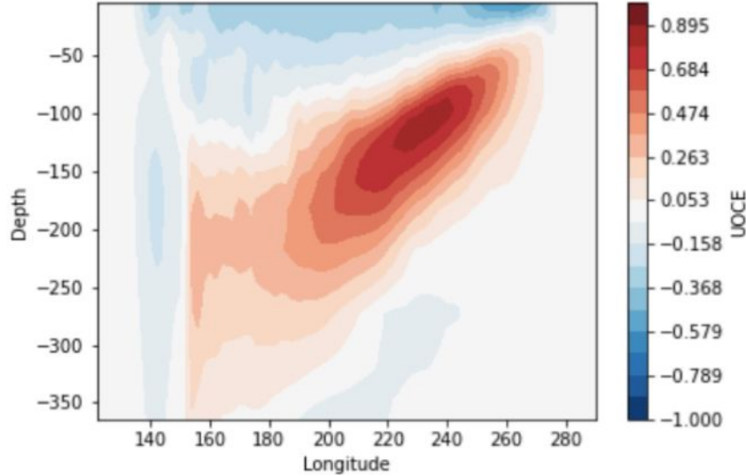
Summer UOCE Profiles at the equator
