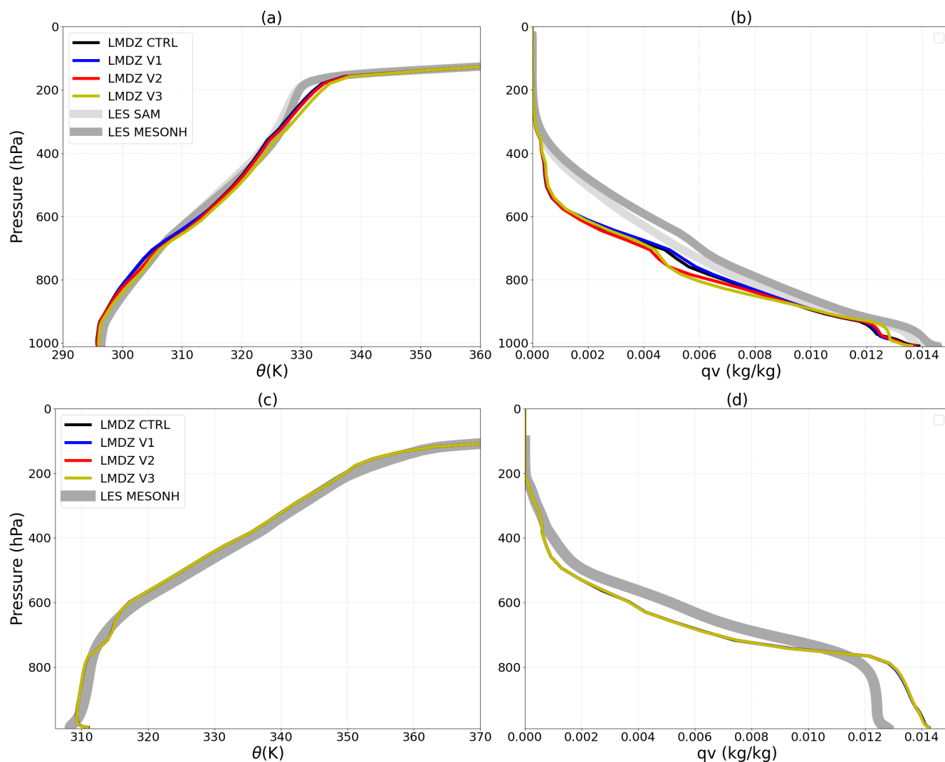
Figure 9. Vertical profiles of potential temperature ( \theta ) and specific humidity ( q_v ) calculated in the LES and simulated with LMDZ: for a control simulation (CTRL), with adjustment of the coefficient k to 0.56 (V1), with the modified computation of p_{upper} (V2) and with the activation of thermals in the entire domain (V3). Both the RCE (a, b) and AMMA (c, d) cases are shown for the same times as in Fig. 7
