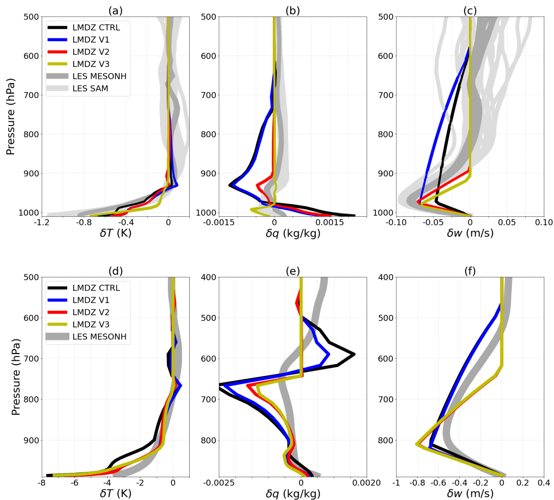
Figure 8. Vertical profiles of \delta T , \delta q and \delta w calculated in the LES and simulated with LMDZ: for a control simulation (CTRL, same curves as Fig. 7), with adjustment of the coefficient k to 0.56 (V1), with the modified computation of p_{upper} (V2) and with the activation of thermals in the entire domain (V3). Both the RCE (a, b, c) and AMMA (d, e, f) cases are shown for the times as in Fig. 9.
