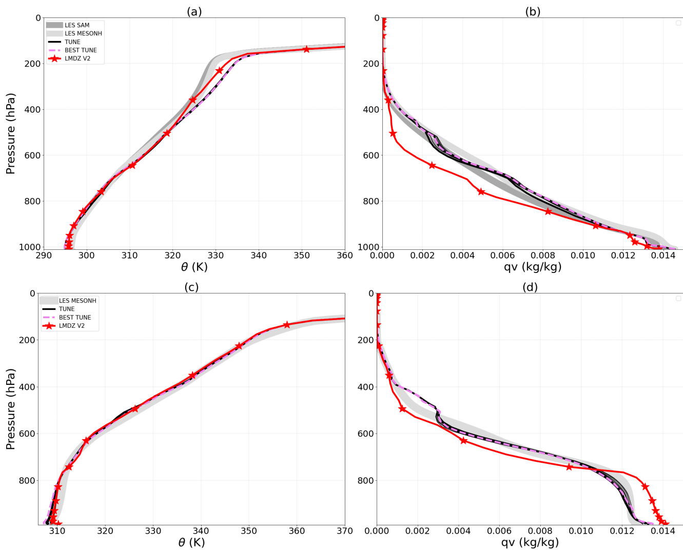
Figure 11. Like Fig. 9, but showing for LMDZ, the V2 simulation, the 12 best simulations from the tuning (TUNE, in black) as well as the best one among them (TUNE BEST, in greenviolet dotted ).
