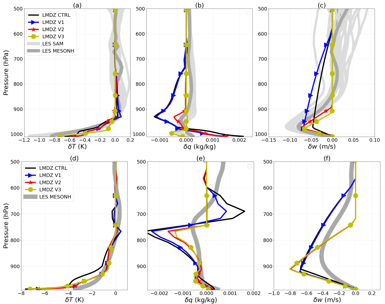
Figure 8. Vertical profiles of \delta T , \delta q , \delta w and \delta w - \delta W calculated in the LES and simulated with LMDZ: for a control simulation (CTRL, same curves as Fig. 7), with adjustment of the coefficient k to 0.56 (V1), with the modified computation of p_{upper} (V2) and with the activation of thermals in the entire domain (V3). Both the RCE (a, b, c) and AMMA (d, e, f) cases are shown for the times as in Fig. 9.
