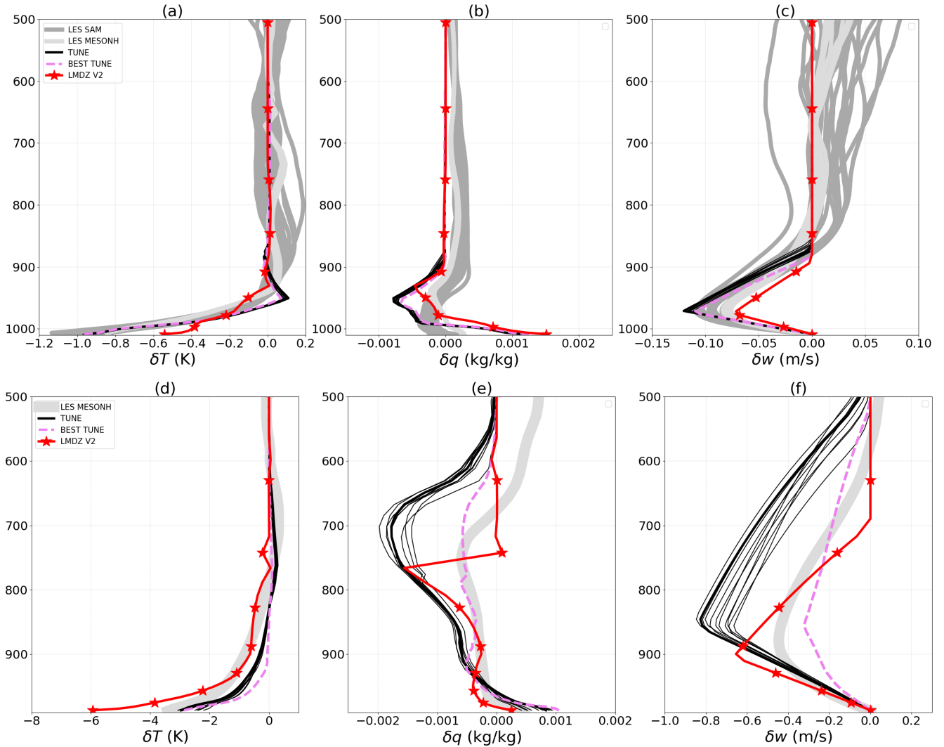
Figure 10. Like Fig. 8, but showing for LMDZ, the V2 simulation, the 12 best simulations from the tuning (TUNE, in black) as well as the best one among them (TUNE BEST, in greenviolet dotted ).
