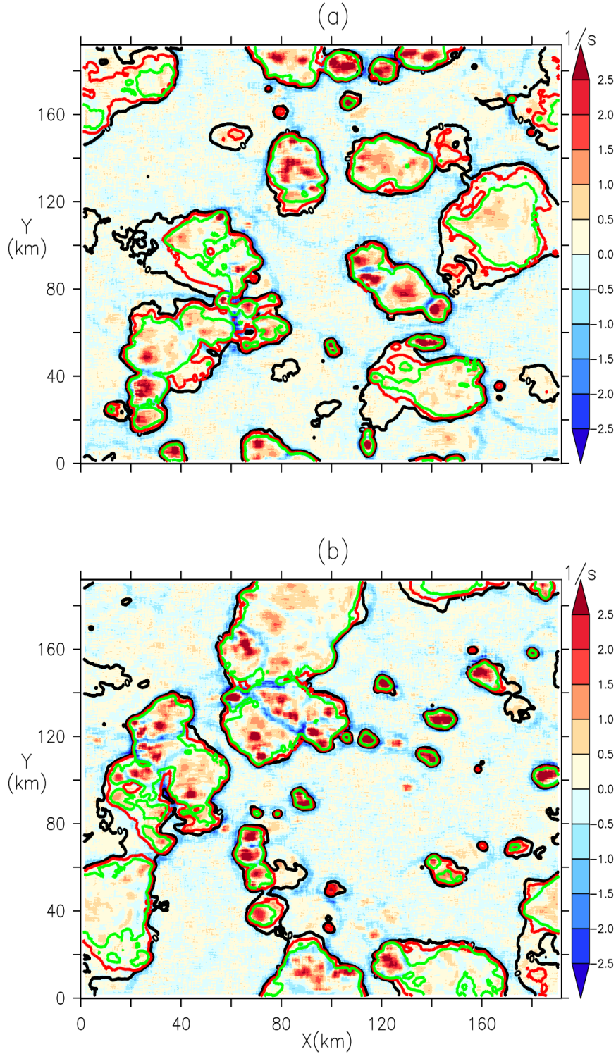
Figure 2: Map Sliding average (with a box of 3.25 \text{ km} \times 3.25 \text{ km} ) of the divergence of wind at 10 m V_{10m} (in s^{-1} 10^{-3} s^{-1} ) multiplied by 1000 and smoothed horizontally over 3.25. Changer l'unité 1/s sur les figures ou l'enlève. With this unit, a value of 1 corresponds to a change of wind intensity of 1 \text{ km} \times 3.25 \text{ m s}^{-1} for 1 km represented on two instants (-). Panels a and b correspond to two different states of the LES SAM carried out on the oceanic RCE case and superimposed with the contours. Contours of temperature anomalies at 10 m at -0.4 K (green), -0.2 K (red) and 0 K (black) are superimposed on the smoothed divergence field.
