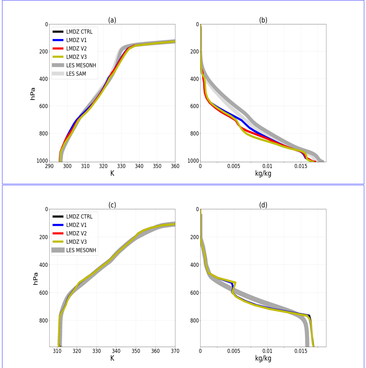
Figure 9: Vertical profiles of potential temperature ( \theta ) and specific humidity ( q_v ) calculated in the LES and simulated in control LMDZ (LMDZ CTRL), LMDZ with the adjustment of the coefficient k to 0.66 (V1), LMDZ with the drop in altitude ( h_m ) at which the subsidence of the air masses in cold pools is zero (V2) and LMDZ with the activation of thermals in the entire domain (V3) on the RCE case (a, b) and on the AMMA case (c, d). The LES profiles correspond simply to horizontal averages over the full domain.
