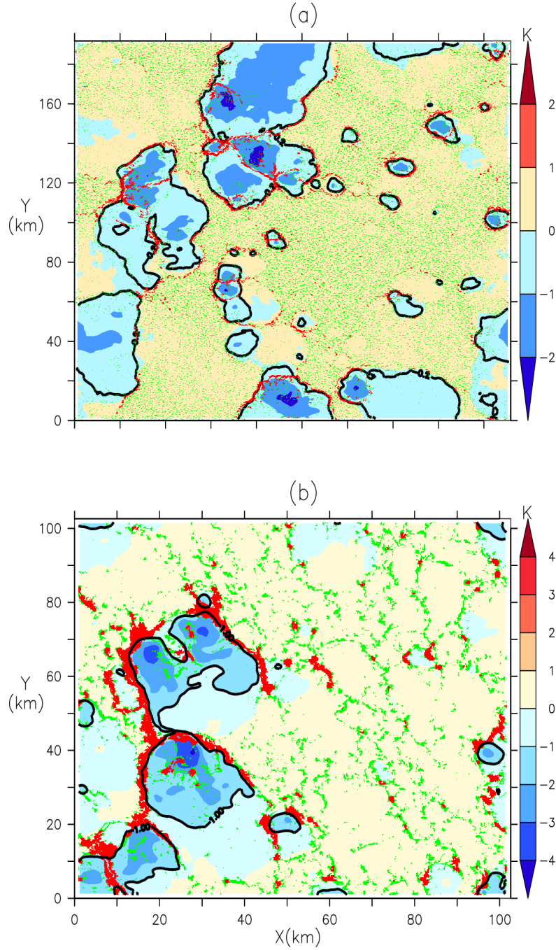
Figure 6: Maps of T_{10m} anomaly of temperature at 10 m, smoothed horizontally over with a sliding average with a horizontal box of 2.5 \text{ km} \times 2.5 \text{ km} , represented on at an instant of the LES SAM of the RCE case (a) and on the instant 6:00 PM of the LES of the AMMA case with black contours indicating thresholds of temperature at 10 m anomaly of -0.2 \text{ K} (RCE) and -1 \text{ K} (AMMA). The red color indicates the updrafts on the gust fronts given by the vertical velocities at cloud base ( w_b ) in the gust fronts mask, which. This mask is determined by defined from a threshold value applied to the sliding average of w_b smoothed horizontally over. For the RCE case, the average is done with a box of 1.25 \text{ km} \times 1.25 \text{ km} and exceeding 0.6 values of \tilde{w}_b > 0.6 \text{ m s}^{-1} are retained (RCE) and over respectively 2 \text{ km} \times 2 \text{ km} with a value greater than 2 and \tilde{w}_b > 2 \text{ m s}^{-1} for AMMA). il manque les valeurs de w_b au dessus des quelles on trace les ponints de grille rouge et vert. The green dots represent thermals, defined by w_b outside the gust front mask.
