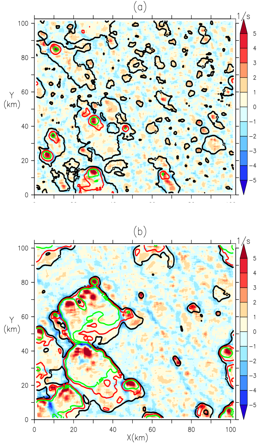
Figure 3: Map of divergence of wind at 10 m (in s^{-1} ) multiplied by 1000 and smoothed horizontally over 3.25 \text{ km} \times 3.25 \text{ km} represented on the Same as Fig. 2 for two successive instants, 17:10 (a) and 18:00 (b) instants, of the LES MESONH carried out on the AMMA case and superimposed with the contours of superimposed corresponds to T_{10m} anomalies of temperature at 10 m at -1 K (green), -0.5 K (red) and 0 K (black).
