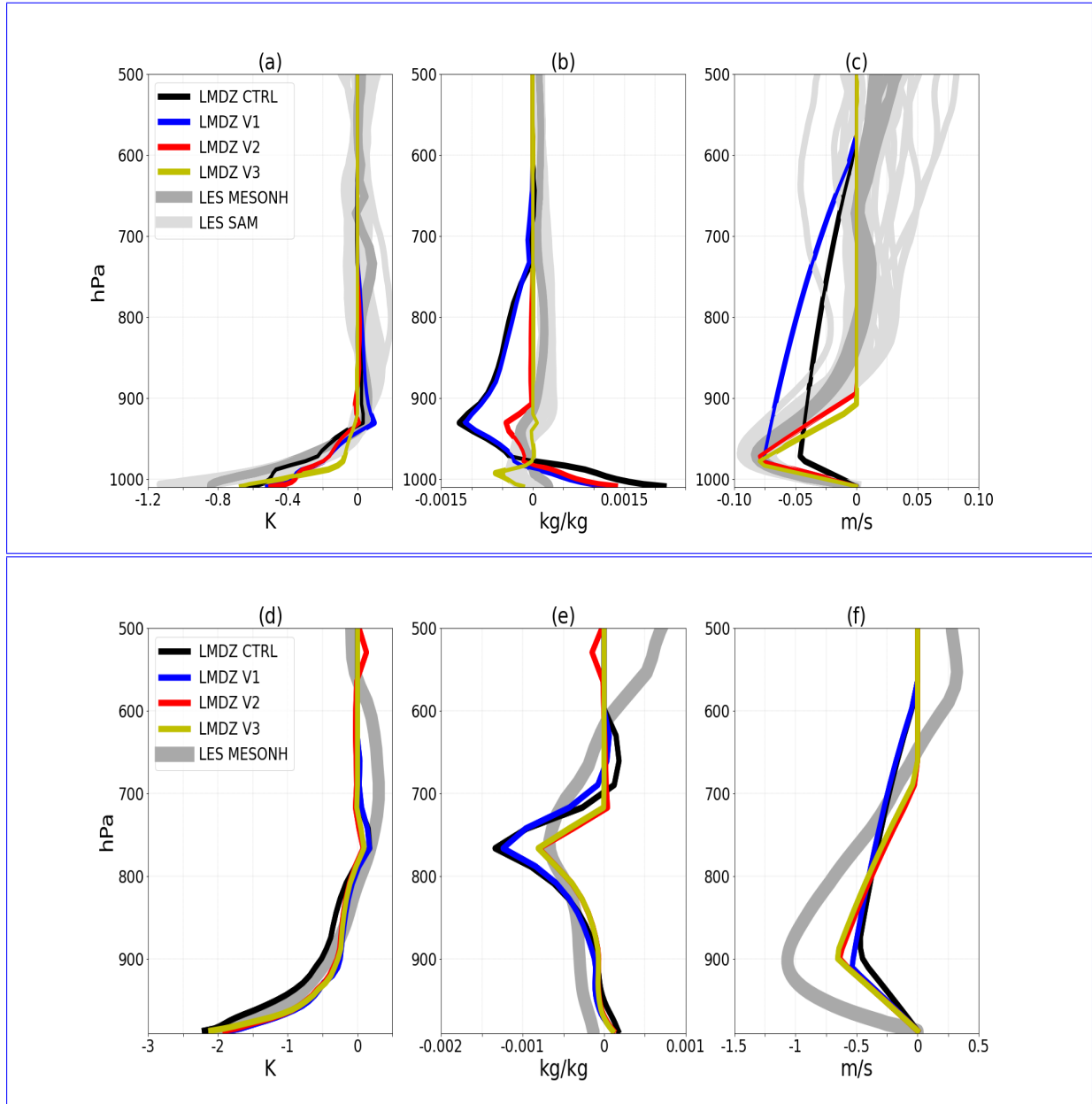
Figure 8: Vertical profiles of \delta T , \delta q and \delta w calculated in the LES and simulated in the control LMDZ (CTRL), LMDZ with the adjustment of the coefficient k to 0.66 (V1), LMDZ with the drop in altitude ( h_m ) at which the subsidence of the air masses in cold pools is zero (V2) and LMDZ with the activation of thermals in the entire domain (V3) on the RCE case (a, b, c) and on the AMMA case (d, e, f).
