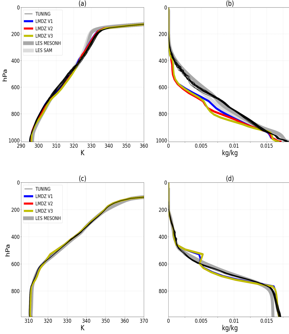
Figure 11: Vertical profiles of potential temperature ( \theta ) and specific humidity ( q ) calculated in the LES and simulated in LMDZ TUNING, with the adjustment of the coefficient k to 0.66 (V1), LMDZ with the drop in altitude ( h_m ) at which the subsidence of the air masses in cold pools is zero (V2) and LMDZ with the activation of thermals in the entire domain (V3) on the RCE case (a, b, c) and on the AMMA case (d, e, f).
