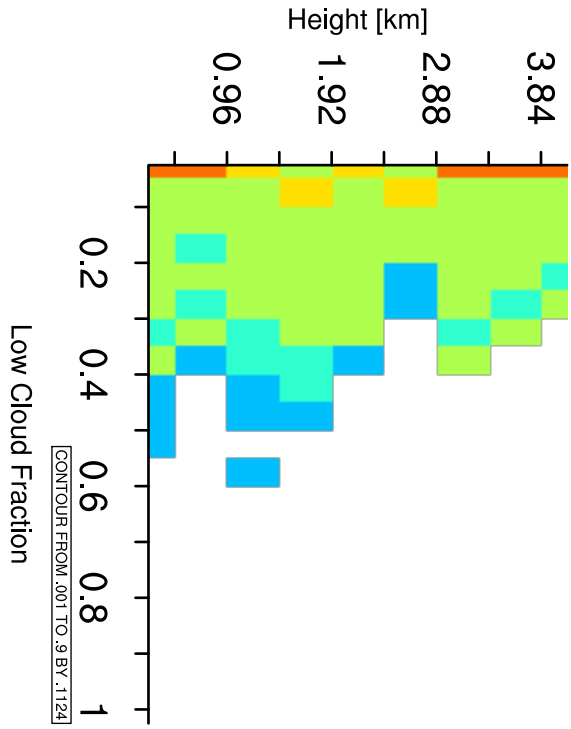
IPSLCM6 Stratocumulus
