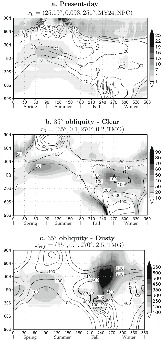
Fig. 3. Latitudinal evolution of the water vapor column (contours, pr. \mu\text{m} ) and water–ice clouds (shaded regions, same unit) as a function of time (in degrees of solar longitude angle L_s ), under present-day (a) and paleoclimatic conditions. (b, c) The predicted water cycle when assuming an equatorial water source and a 35° obliquity, under low dust ( \tau_{dust} = 0.2 ) and high dust ( \tau_{dust} = 2.5 ) conditions, respectively. Water sources are indicated by the acronyms NPC (Northern Polar Cap) and TMG (Tropical Mountain Glaciers). MY24 stands for Martian Year 24 (1999–2000).
