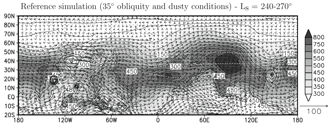
Fig. 6. Average cloud ice content (shaded regions, pr. \mu\text{m} ) and horizontal wind field at the 5.6-km level ( \text{m s}^{-1} ). White lines indicate water vapor column (pr. \mu\text{m} ).
