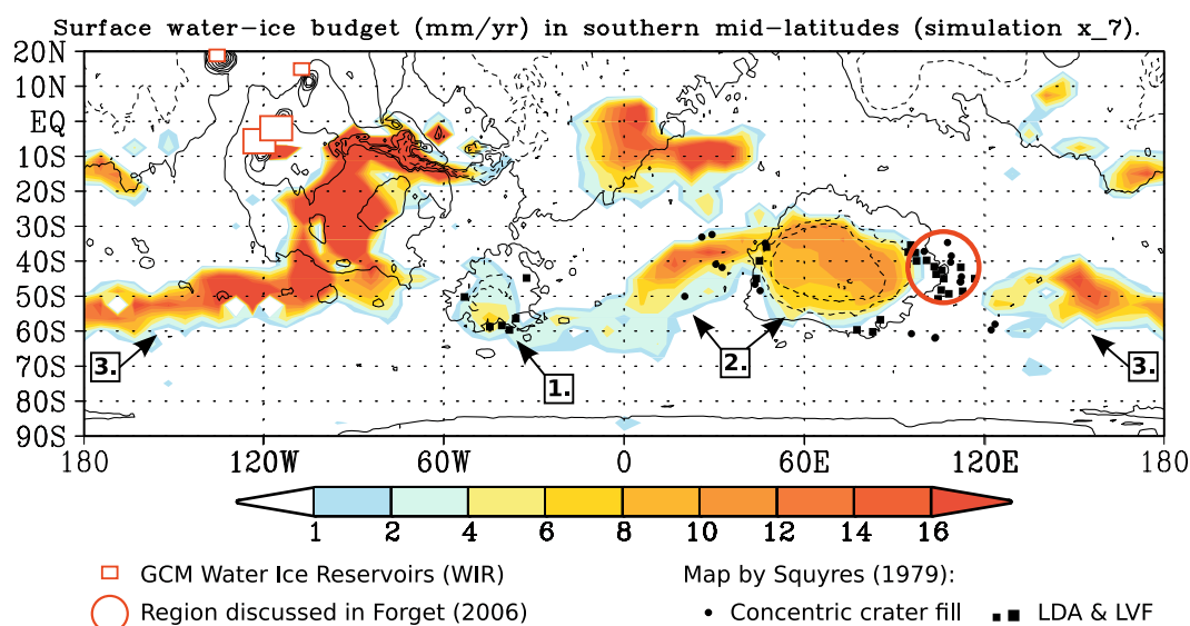
Fig. 10. Net ice accumulation ( mm\ yr^{-1} ) predicted in simulation x_7 = (35^\circ, 0.1, 90^\circ, 2.5, TMG) , superposed on the map by Squyres (1979). LDA and LVF stand for Lobate Debris Aprons and Lineated Valley Fill. Indicated regions: 1. Argyre Planitia, 2. Western Hellas, 3. Terra Sirenum (left), and Terra Cimmeria (right).
