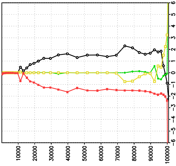
tendencies, beta=1., LMDZ5B physiq
