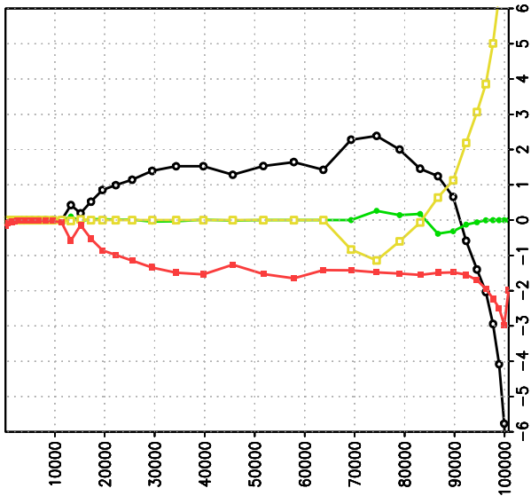
tendencies, beta=0.1, LMDZ5B physiq
