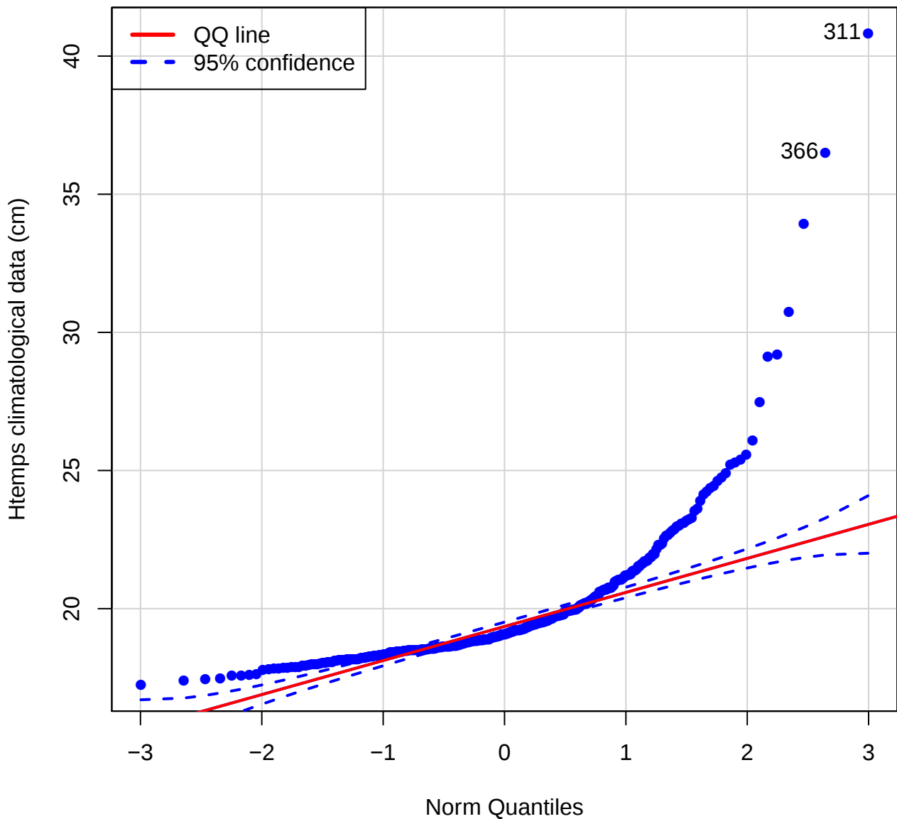
QQ plot (Htemps of LAMC)
