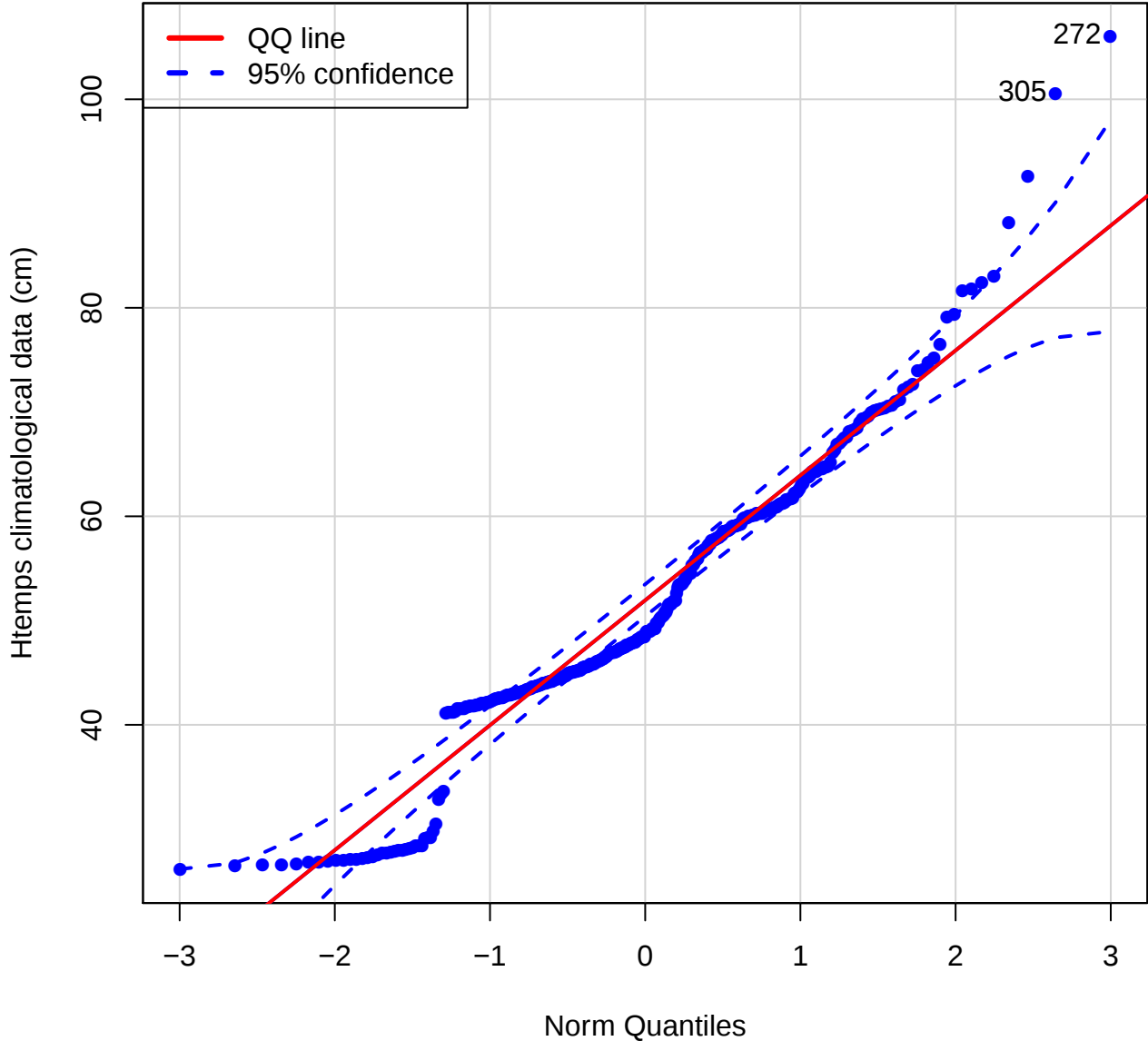
QQ plot (Htemps of LAML)
