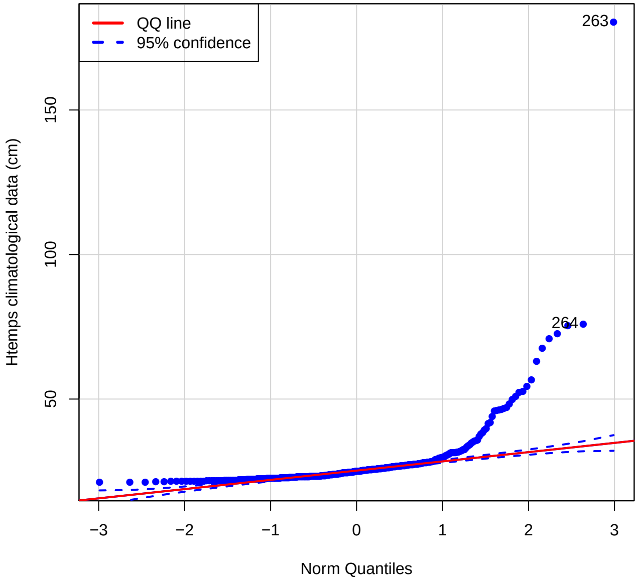
QQ plot (Htemps of LAMM)
