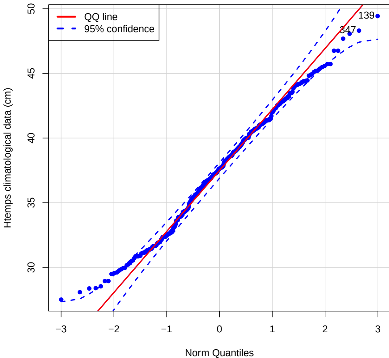
QQ plot (Htemps of STJS)
