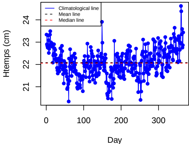
Climatology (FDFB)
