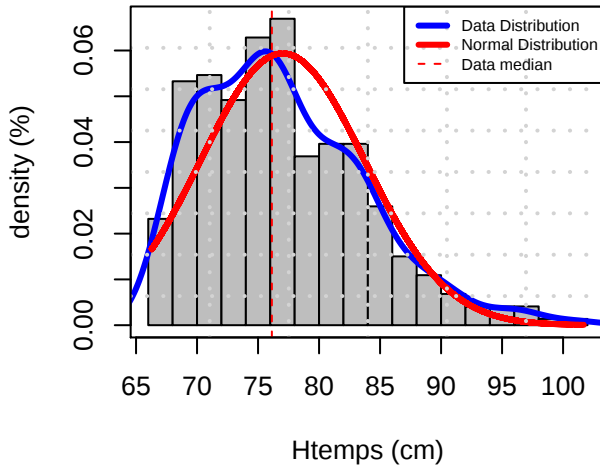
Histogram Distribution (GMPL)
