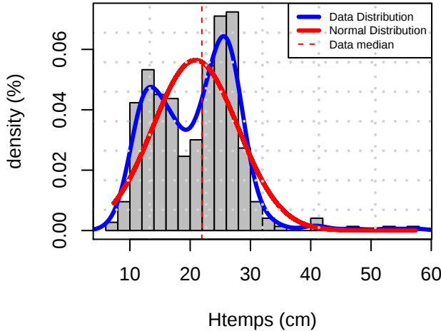
Histogram Distribution (LAMG)
