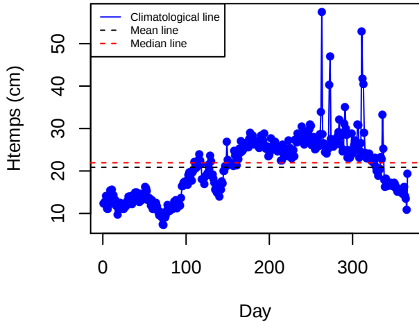
Climatology (LAMG)
