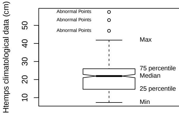
Box plot (LAMG)
