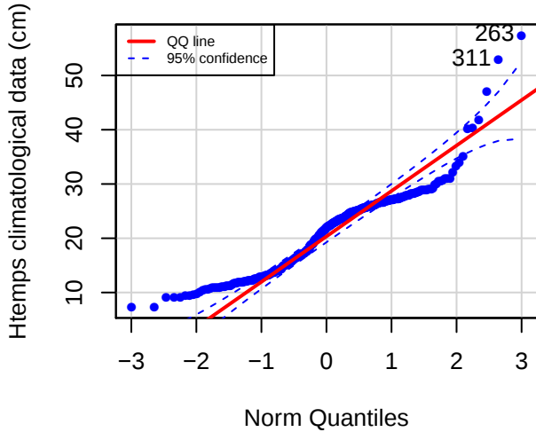
QQ plot (LAMG)
