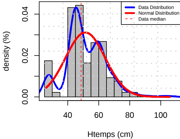
Histogram Distribution (LAML)
