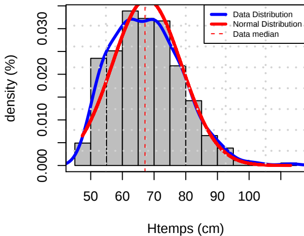
Histogram Distribution (LAMP)
