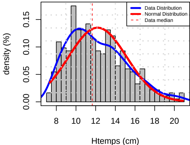
Histogram Distribution (STJA)
