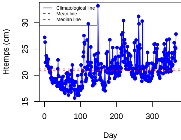
Climatology (STJB)
