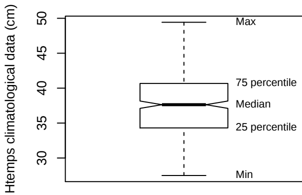
Box plot (STJS)
