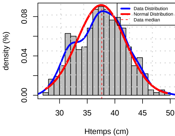
Histogram Distribution (STJS)
