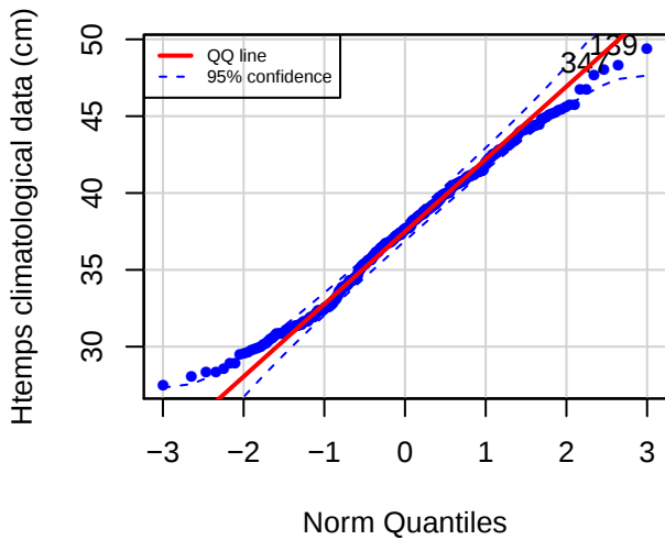
QQ plot (STJS)
