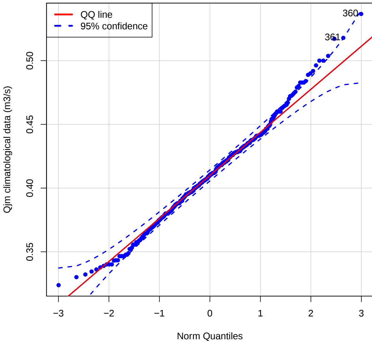
QQ plot (Htemps of FDFB)
