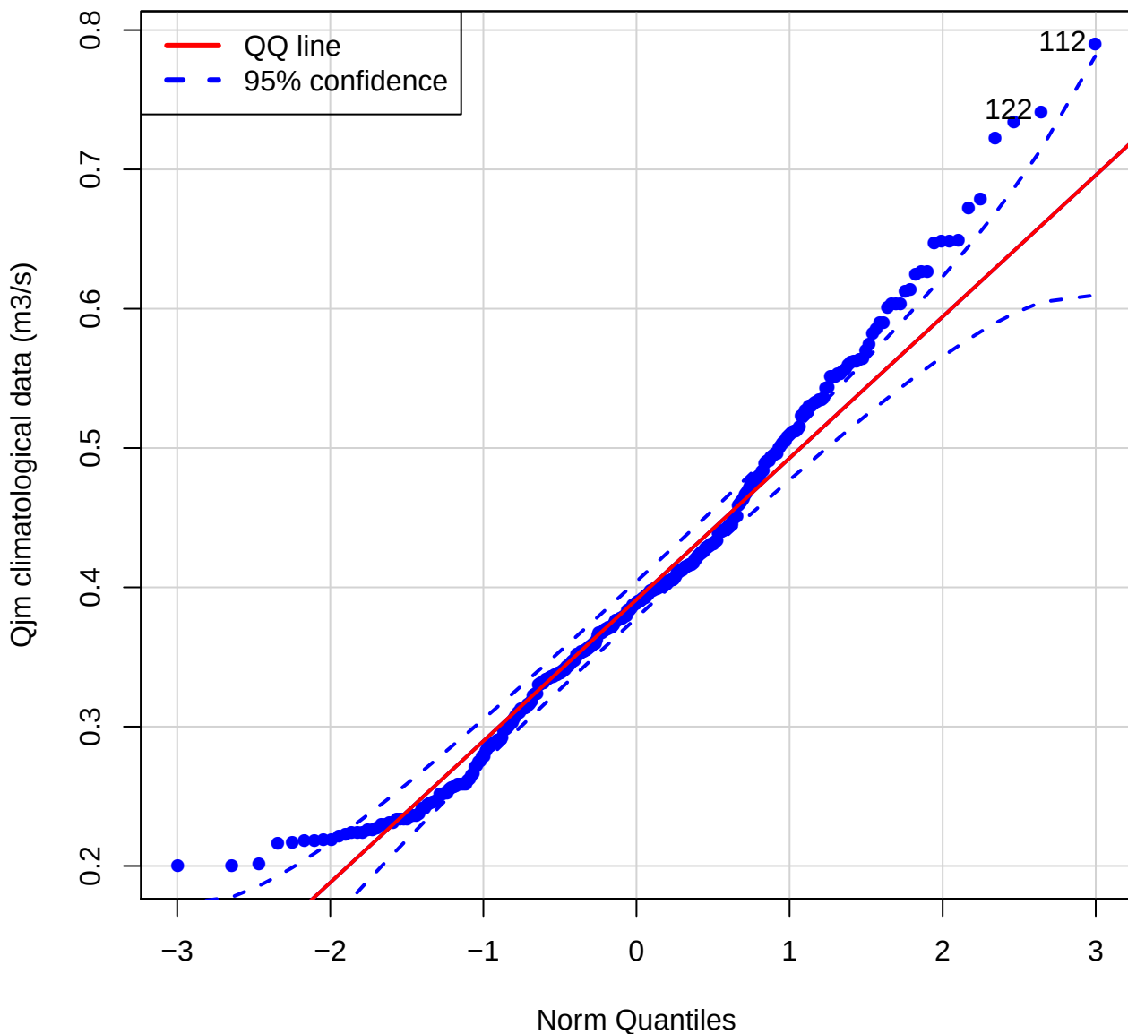
QQ plot (Htemps of GMLP)
