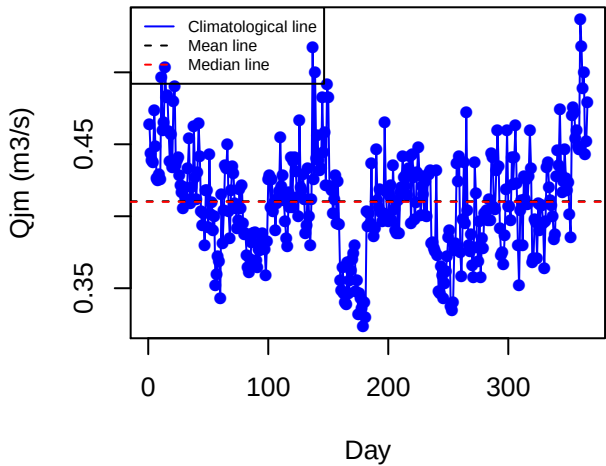
Climatology (FDFB)
