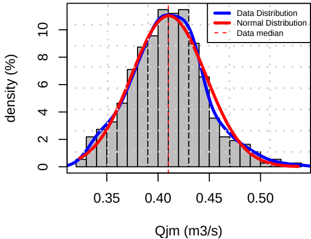
Histogram Distribution (FDFB)
