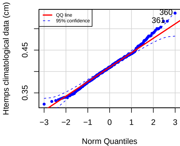
QQ plot (FDFB)
