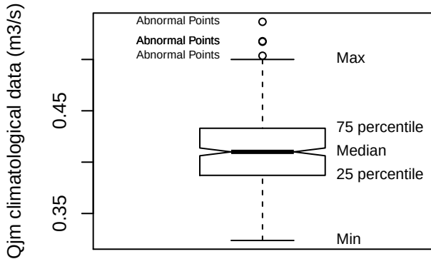
Box plot (FDFB)
