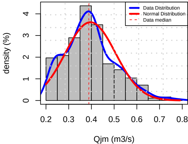
Histogram Distribution (GMLP)
