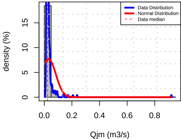
Histogram Distribution (LAMC)
