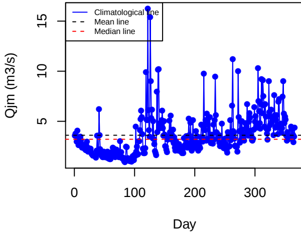
Climatology (LAMP)
