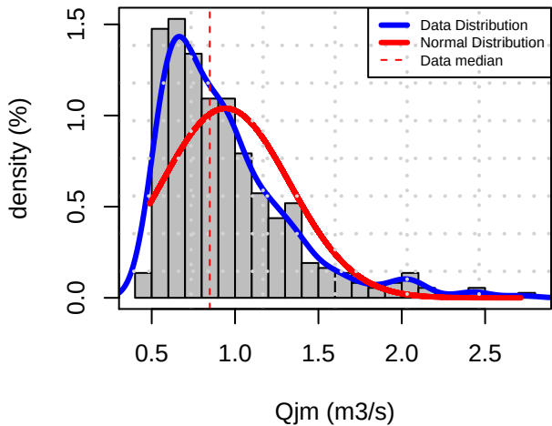
Histogram Distribution (STJA)
