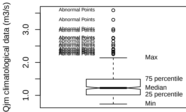
Box plot (STJB)
