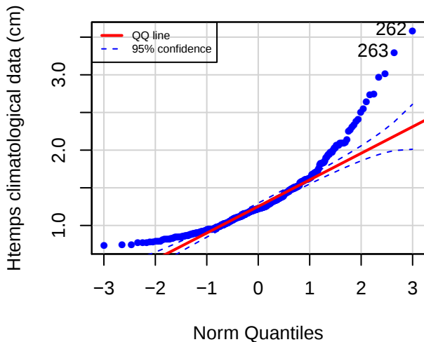
QQ plot (STJB)
