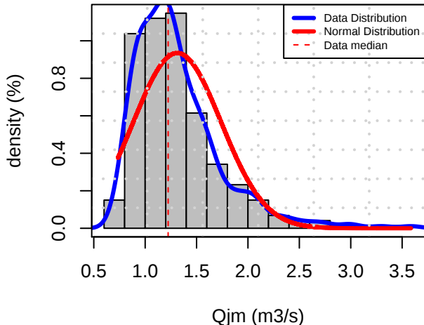
Histogram Distribution (STJB)
