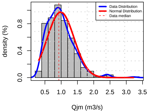
Histogram Distribution (STJS)
