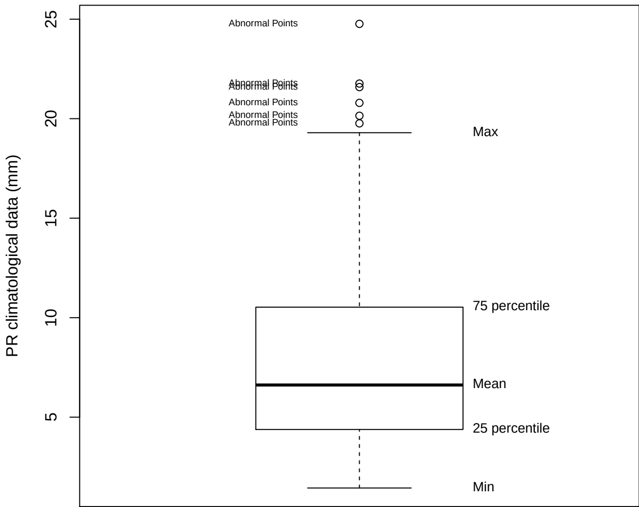
Box plot (PR of BASP)
