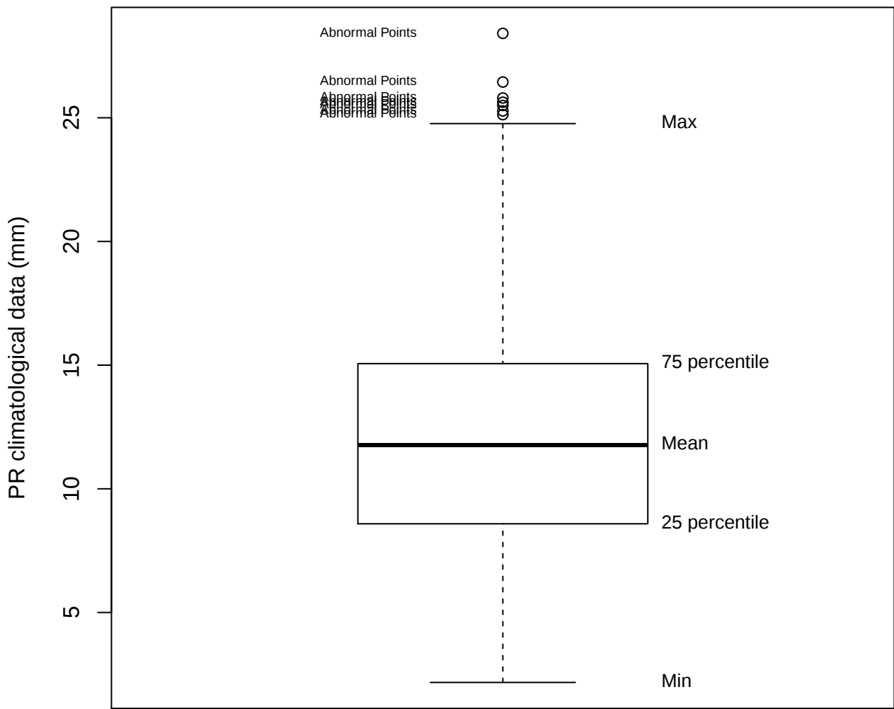
Box plot (PR of FSDG)
