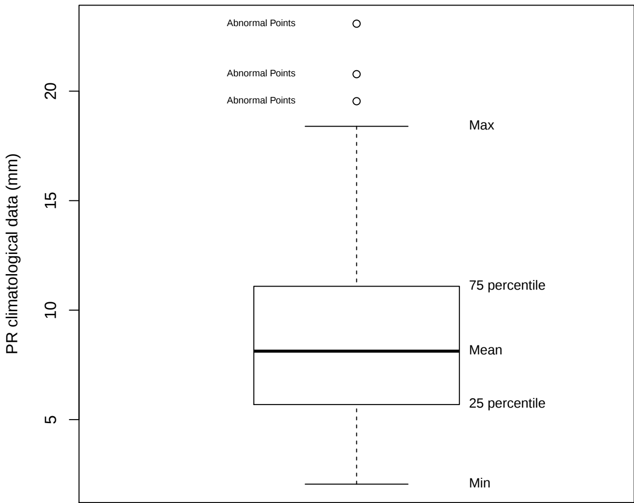
Box plot (PR of STJR)
