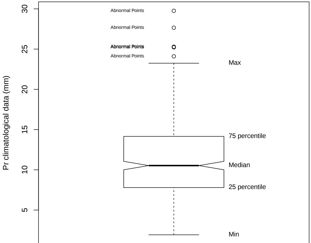
Box plot (Pr of FDFC)
