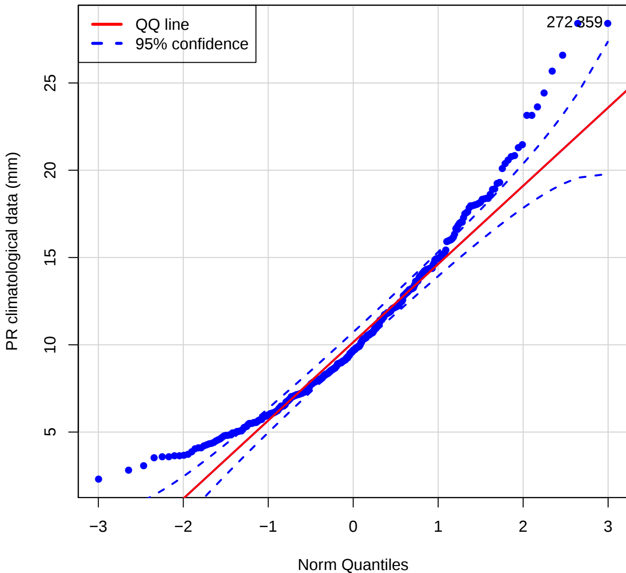
QQ plot (Pr of AJPB)
