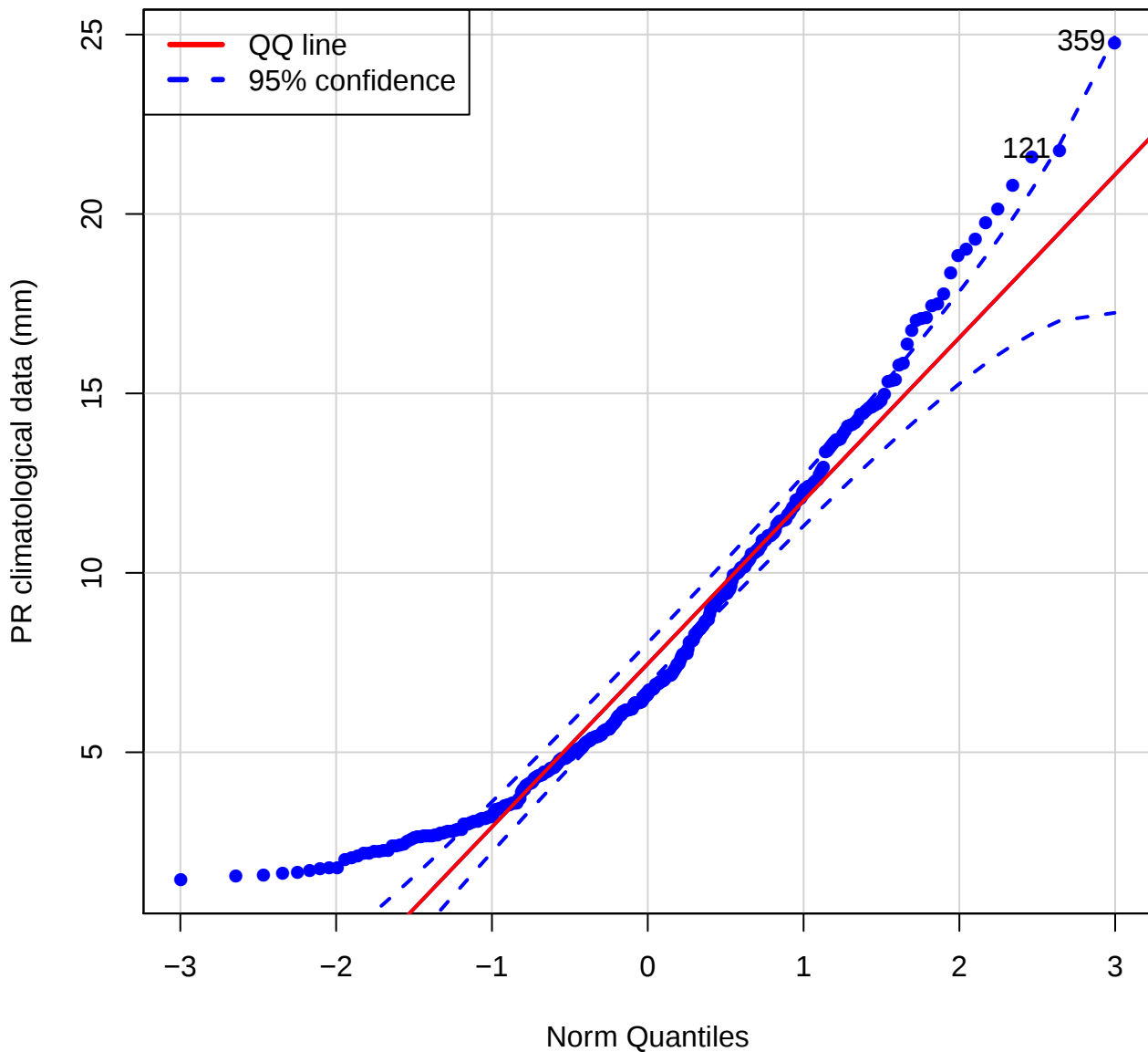
QQ plot (Pr of BASP)
