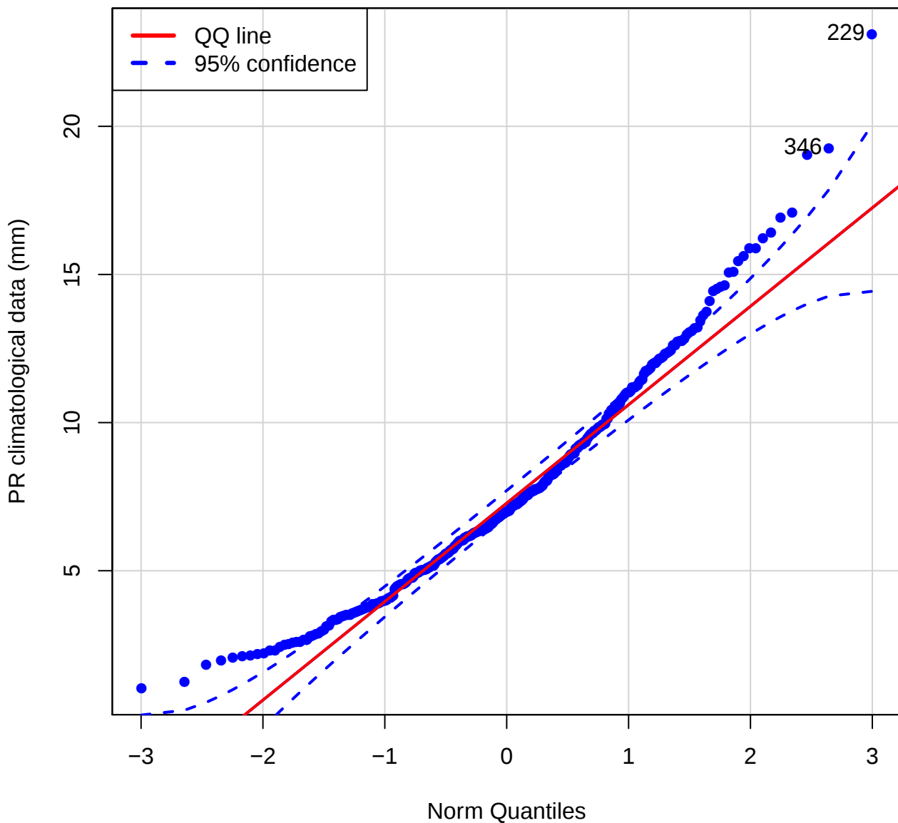
QQ plot (Pr of BLLF)
