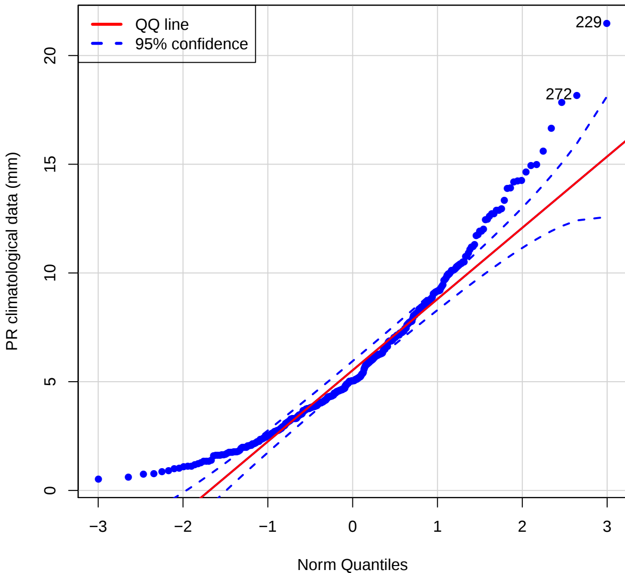
QQ plot (Pr of CARB)
