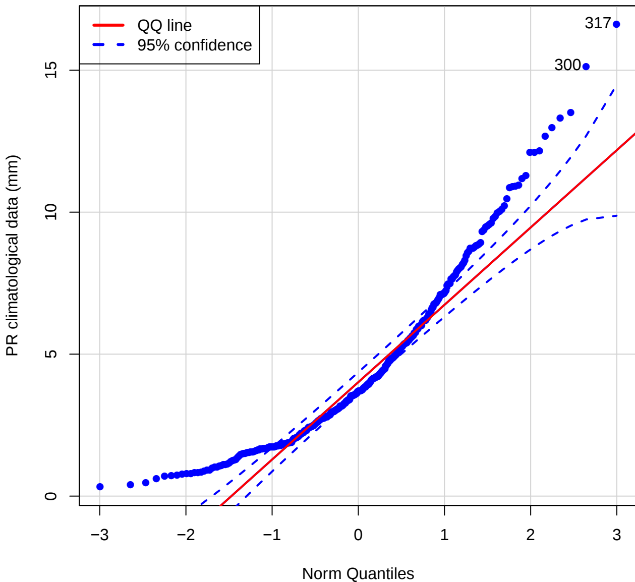
QQ plot (Pr of DIAM)
