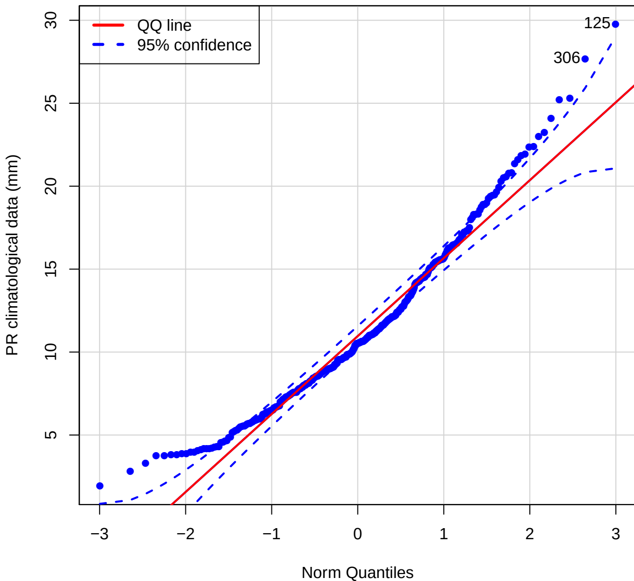
QQ plot (Pr of FDFC)
